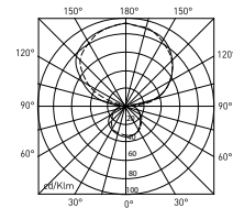
D41B/40.40 - Light intensity distribution
