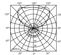
D41/40.40 - Light intensity distribution
