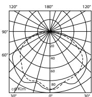
D41/40.40 - Light intensity distribution
