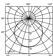
D41B/40.40 - Light intensity distribution
